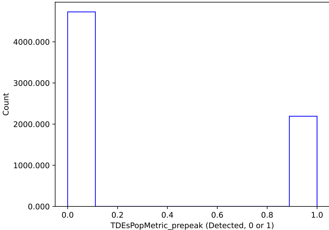
ddf_loaded_fl4_v3.4_10yrs : TDEsPopMetric_prepeak
