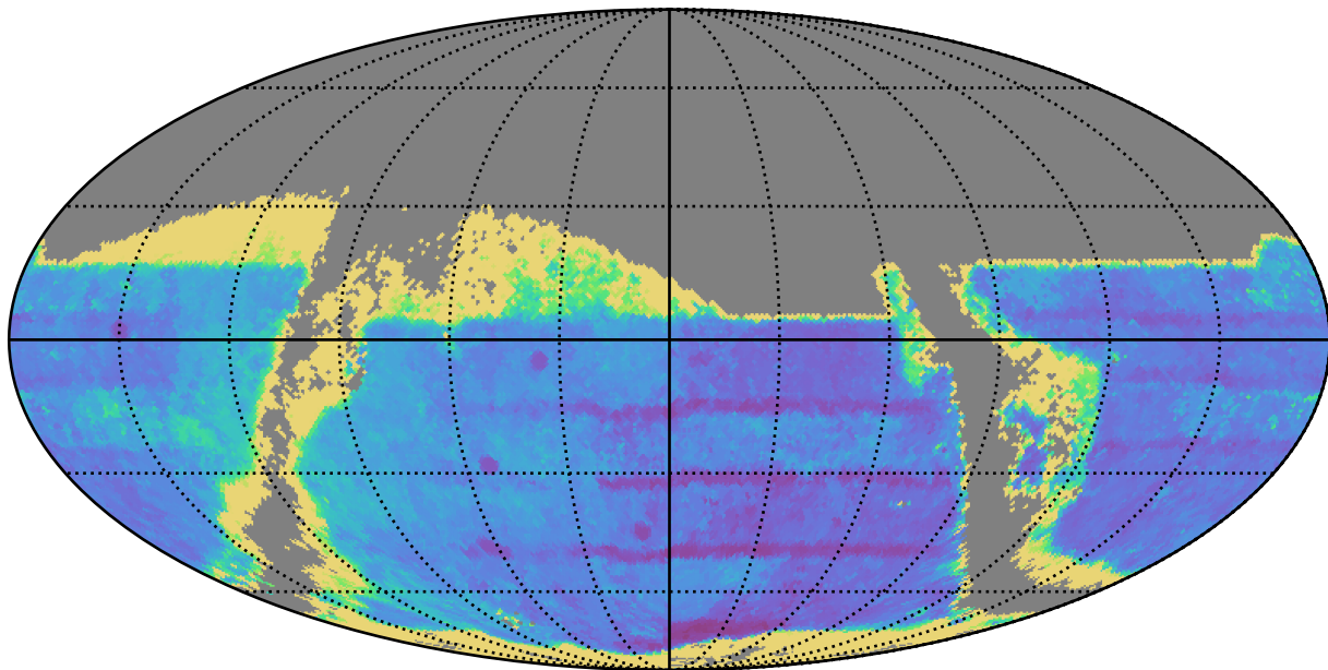
ddf_loaded_fl4_v3.4_10yrs : TDC_accuracy
