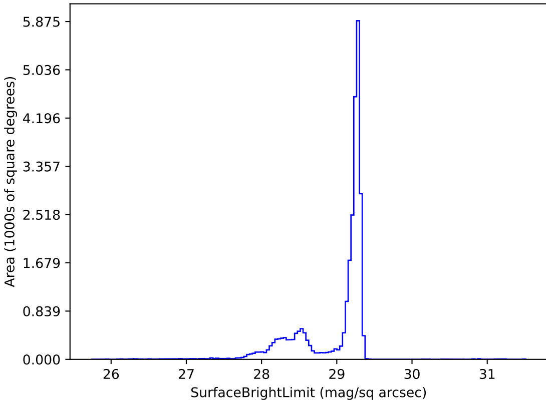
ddf_loaded_fl4_v3.4_10yrs z: SurfaceBrightLimit
