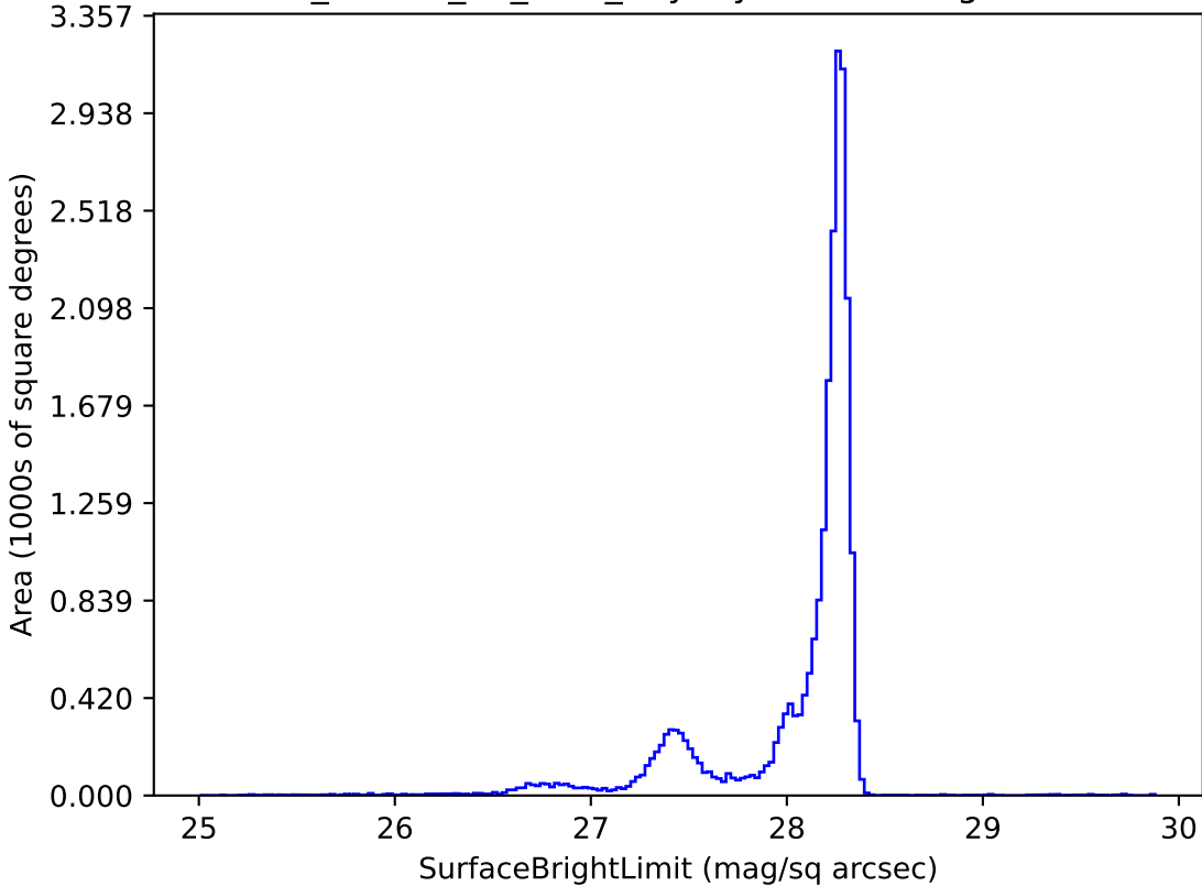
ddf_loaded_fl4_v3.4_10yrs y: SurfaceBrightLimit
