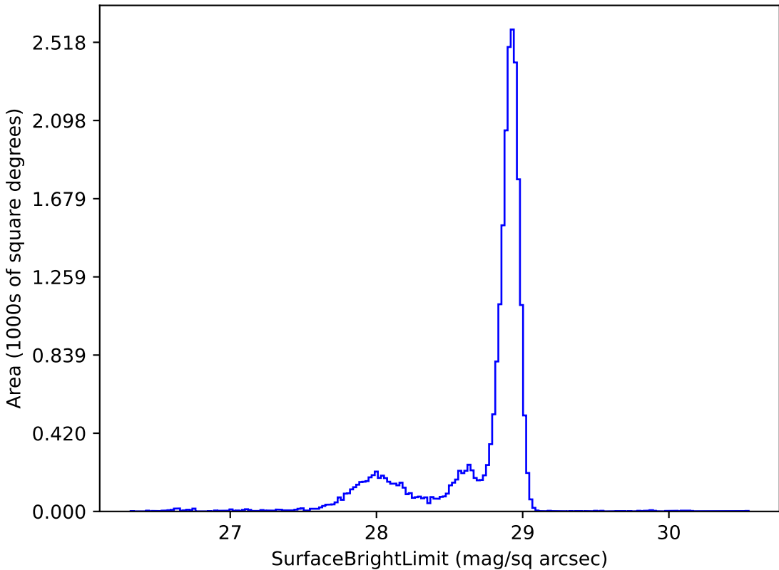
ddf_loaded_fl4_v3.4_10yrs u: SurfaceBrightLimit
