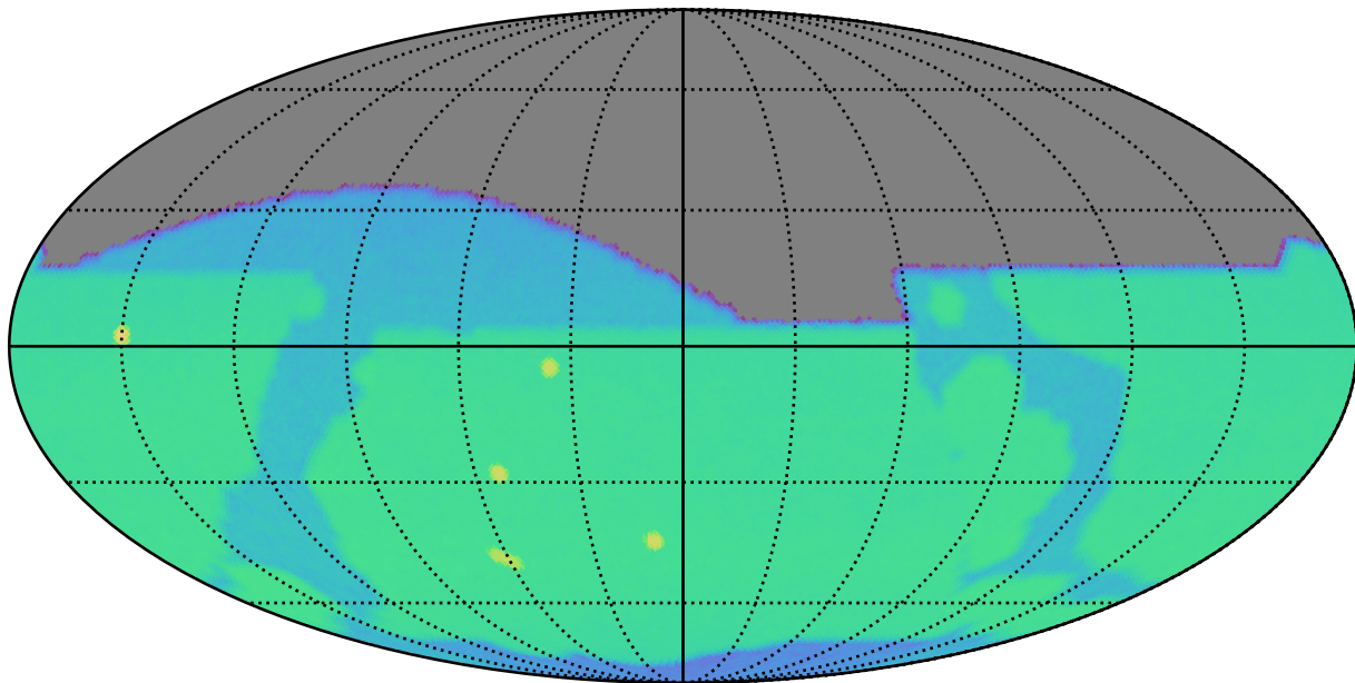
ddf_loaded_fl4_v3.4_10yrs r: SurfaceBrightLimit
