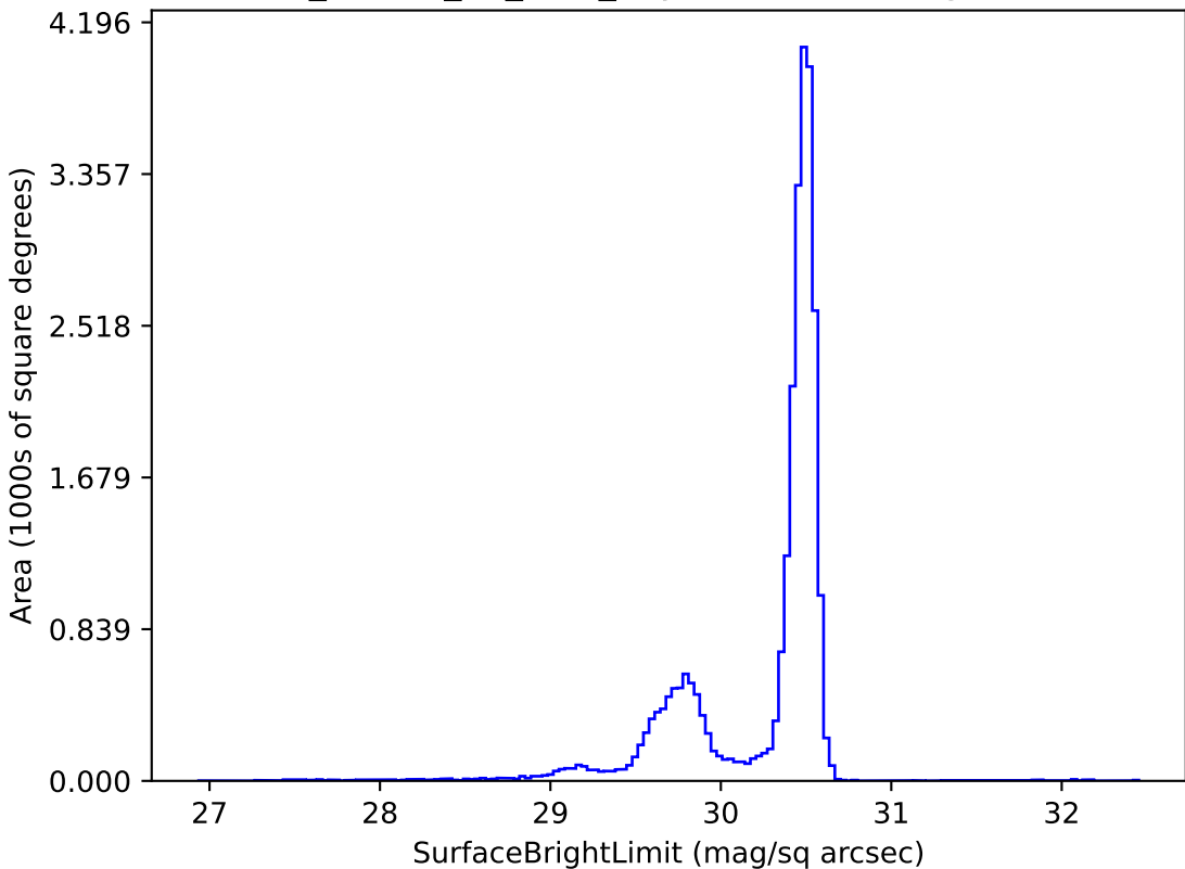
ddf_loaded_fl4_v3.4_10yrs r: SurfaceBrightLimit
