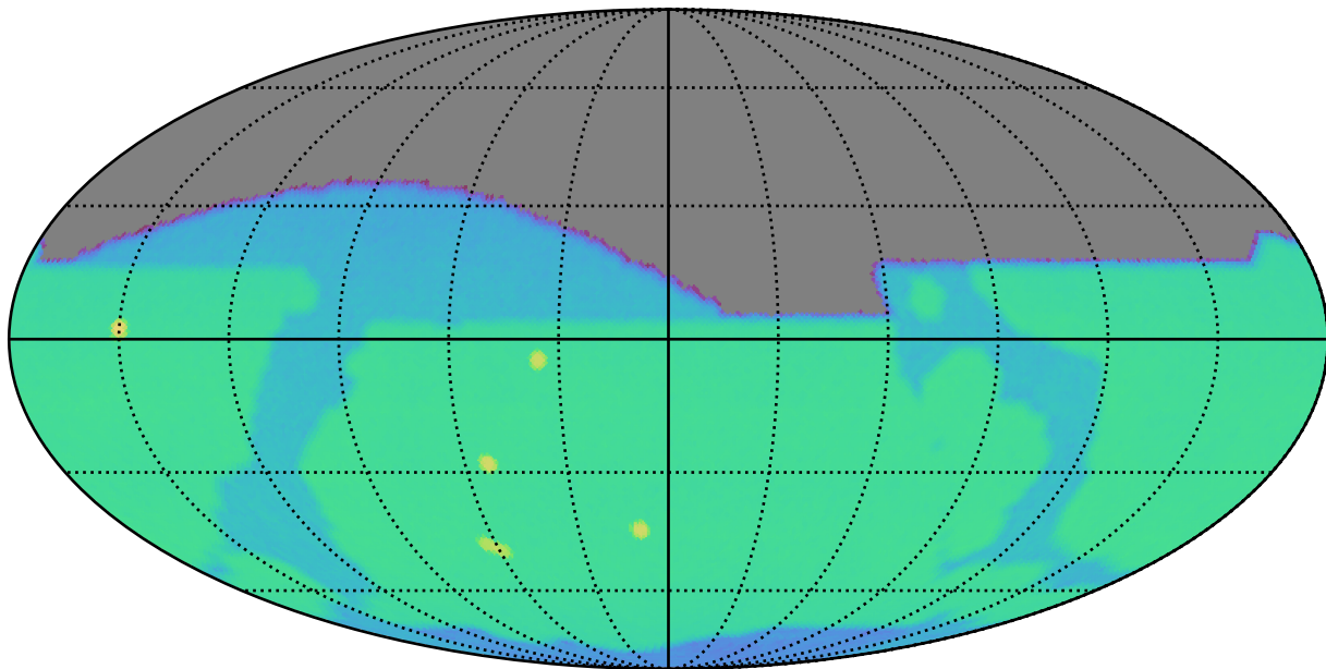
ddf_loaded_fl4_v3.4_10yrs i: SurfaceBrightLimit
