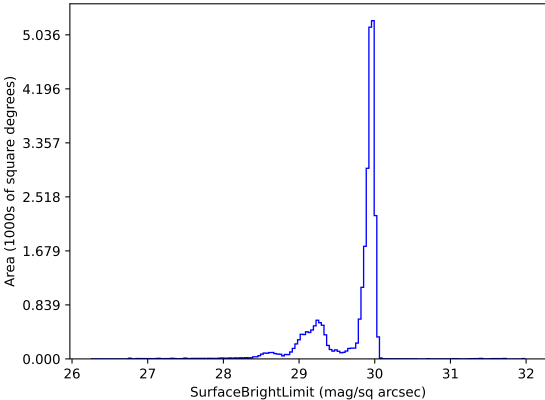
ddf_loaded_fl4_v3.4_10yrs i: SurfaceBrightLimit
