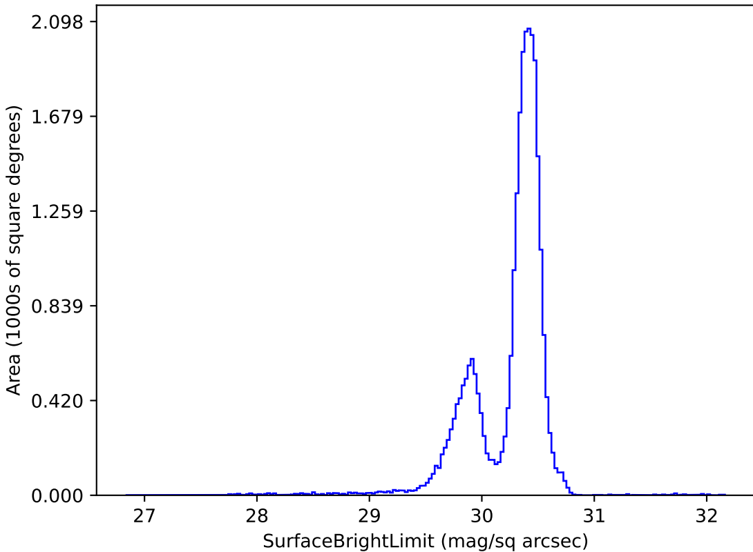
ddf_loaded_fl4_v3.4_10yrs g: SurfaceBrightLimit
