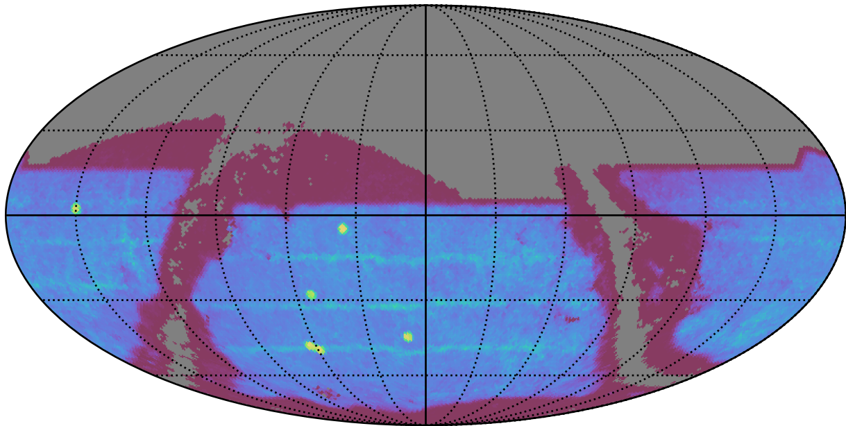
ddf_loaded_fl4_v3.4_10yrs : SNSLMetric
