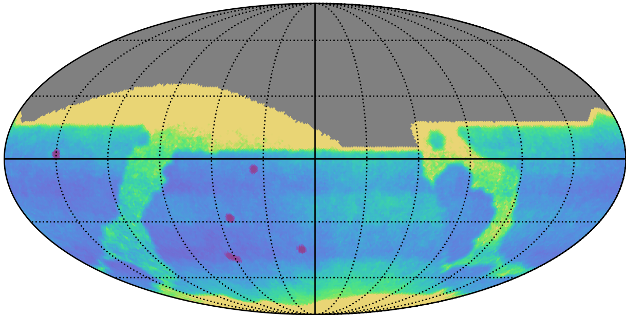
ddf_loaded_fl4_v3.4_10yrs : Proper Motion Uncert @ 24.0
