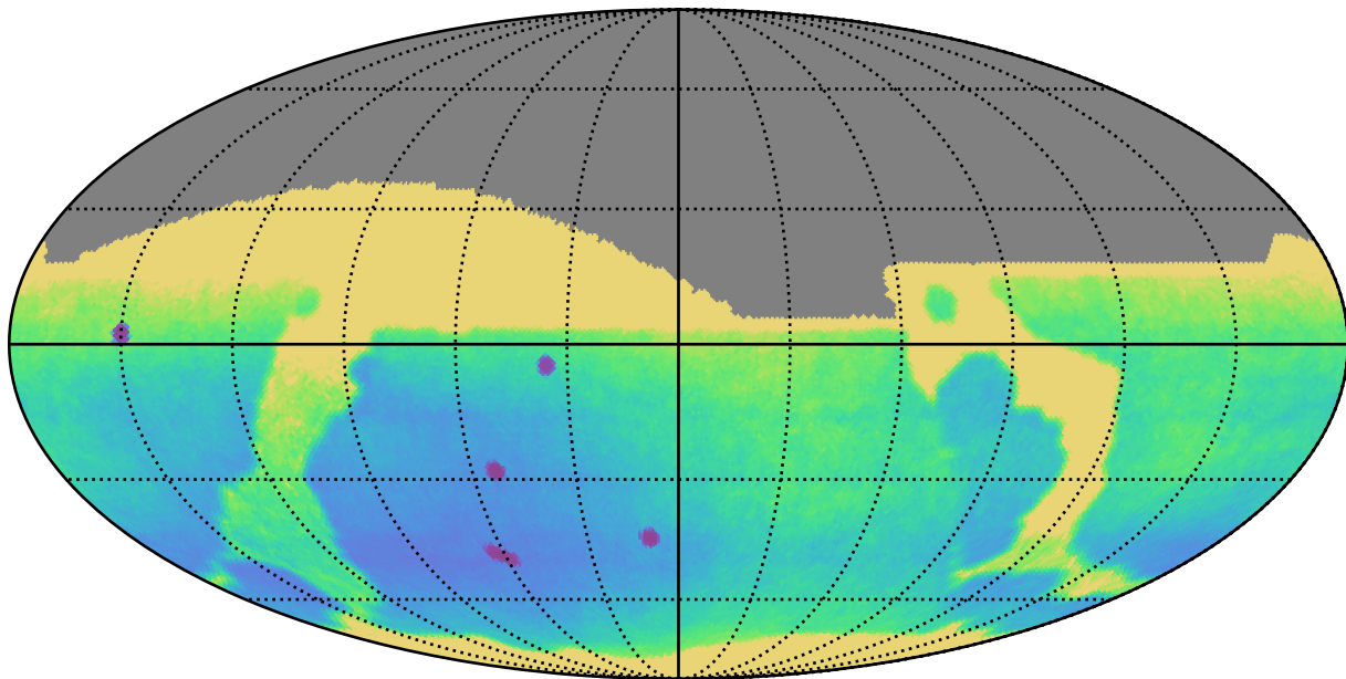
ddf_loaded_fl4_v3.4_10yrs : Parallax Uncert @ 24.0
