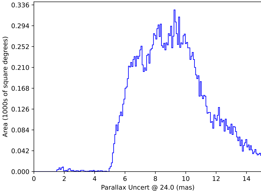
ddf_loaded_fl4_v3.4_10yrs : Parallax Uncert @ 24.0
