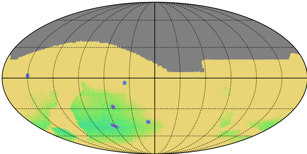
ddf_loaded_fl4_v3.4_10yrs : Parallax Uncert @ 22.4
