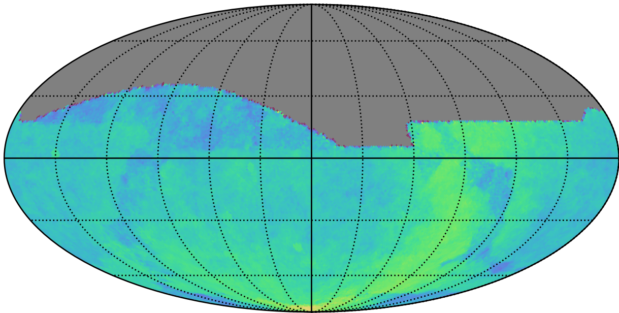
ddf_loaded_fl4_v3.4_10yrs : Parallax Coverage @ 24.0
