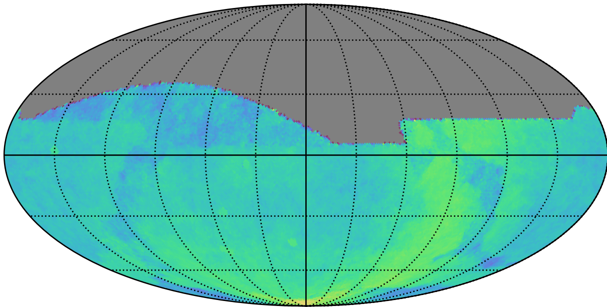
ddf_loaded_fl4_v3.4_10yrs : Parallax Coverage @ 22.4
