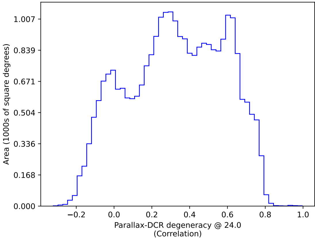
ddf_loaded_fl4_v3.4_10yrs : Parallax-DCR degeneracy @ 24.0
