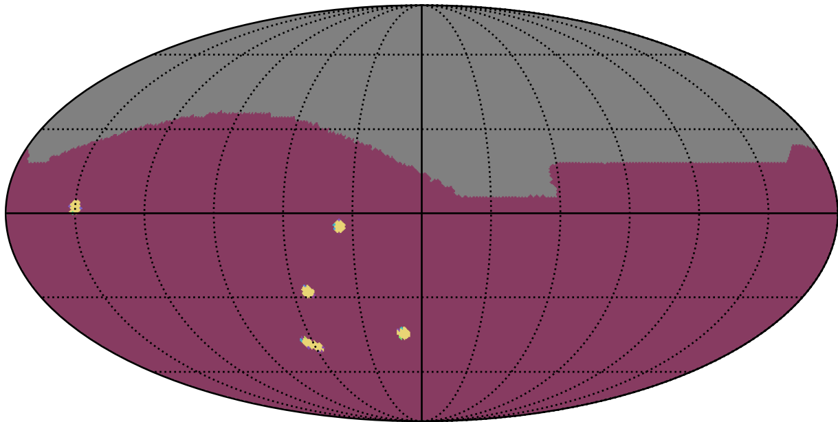
ddf_loaded_fl4_v3.4_10yrs : NumberOfQuickRevisits
