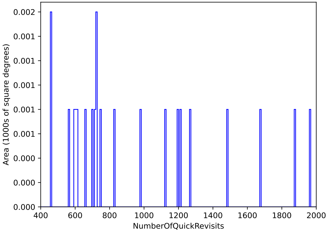
ddf_loaded_fl4_v3.4_10yrs : NumberOfQuickRevisits
