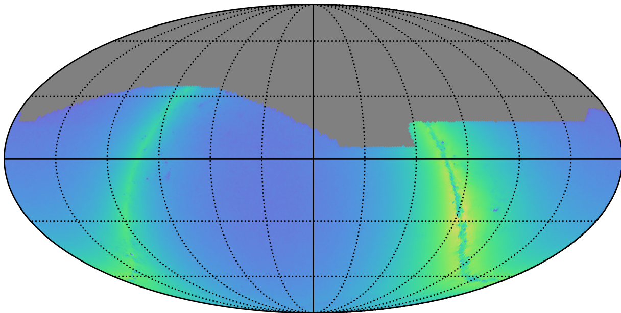
ddf_loaded_fl4_v3.4_10yrs i: Nstars_no_crowding
