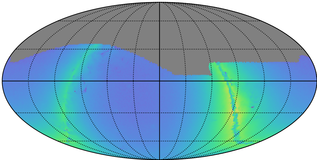
ddf_loaded_fl4_v3.4_10yrs g: Nstars_no_crowding
