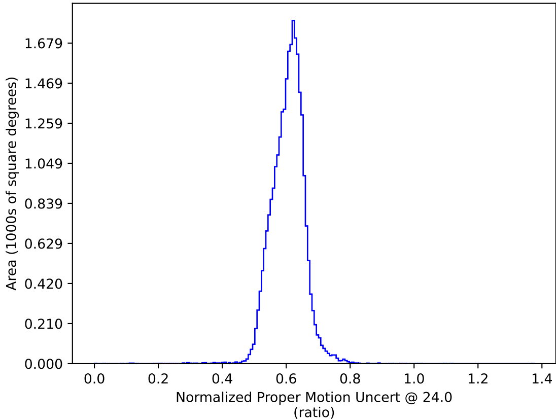
ddf_loaded_fl4_v3.4_10yrs : Normalized Proper Motion Uncert @ 24.0
