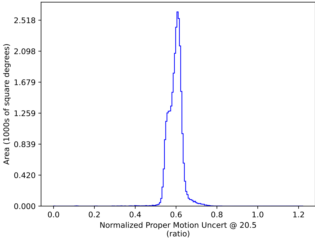
ddf_loaded_fl4_v3.4_10yrs : Normalized Proper Motion Uncert @ 20.5
