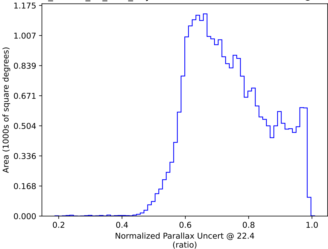
ddf_loaded_fl4_v3.4_10yrs : Normalized Parallax Uncert @ 22.4
