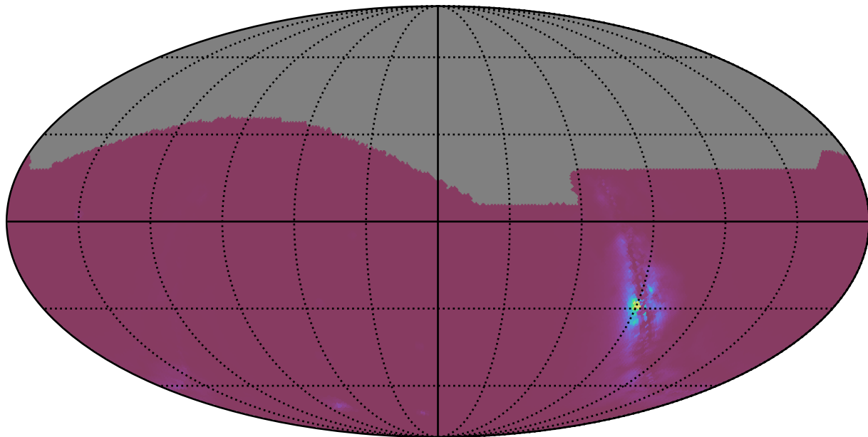
ddf_loaded_fl4_v3.4_10yrs : NlcPoints
