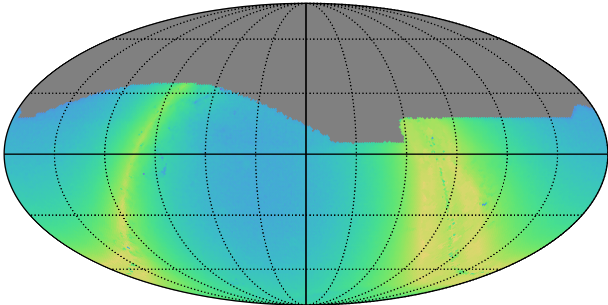
ddf_loaded_fl4_v3.4_10yrs r: N stars to Precision 0.20
