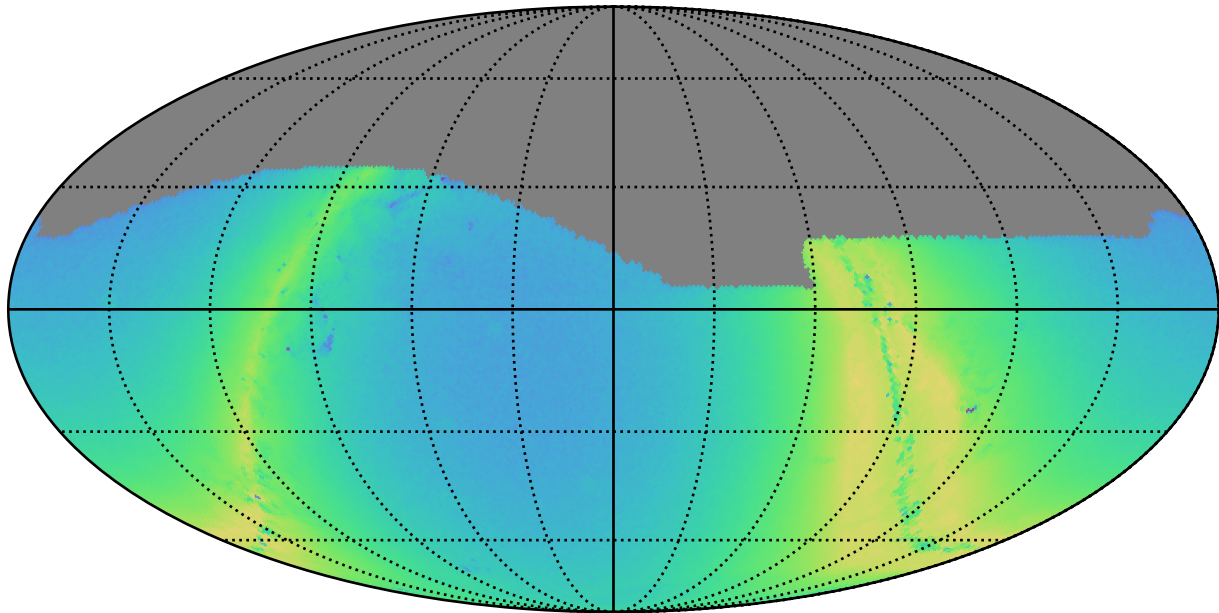
ddf_loaded_fl4_v3.4_10yrs g: N stars to Precision 0.20
