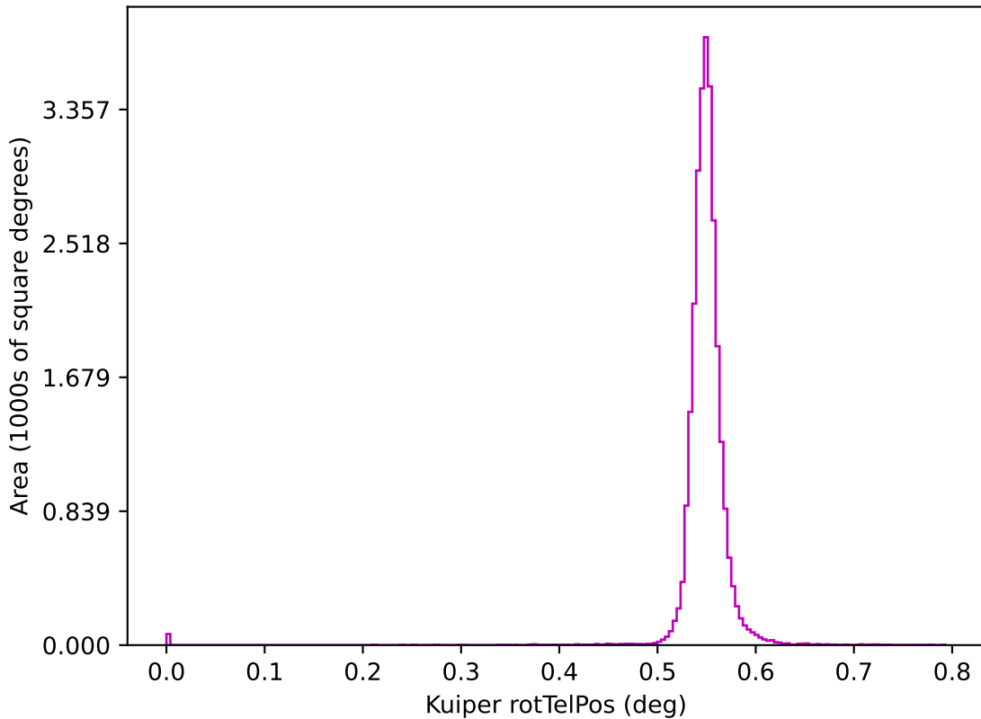
ddf_loaded_fl4_v3.4_10yrs z: Kuiper rotTelPos
