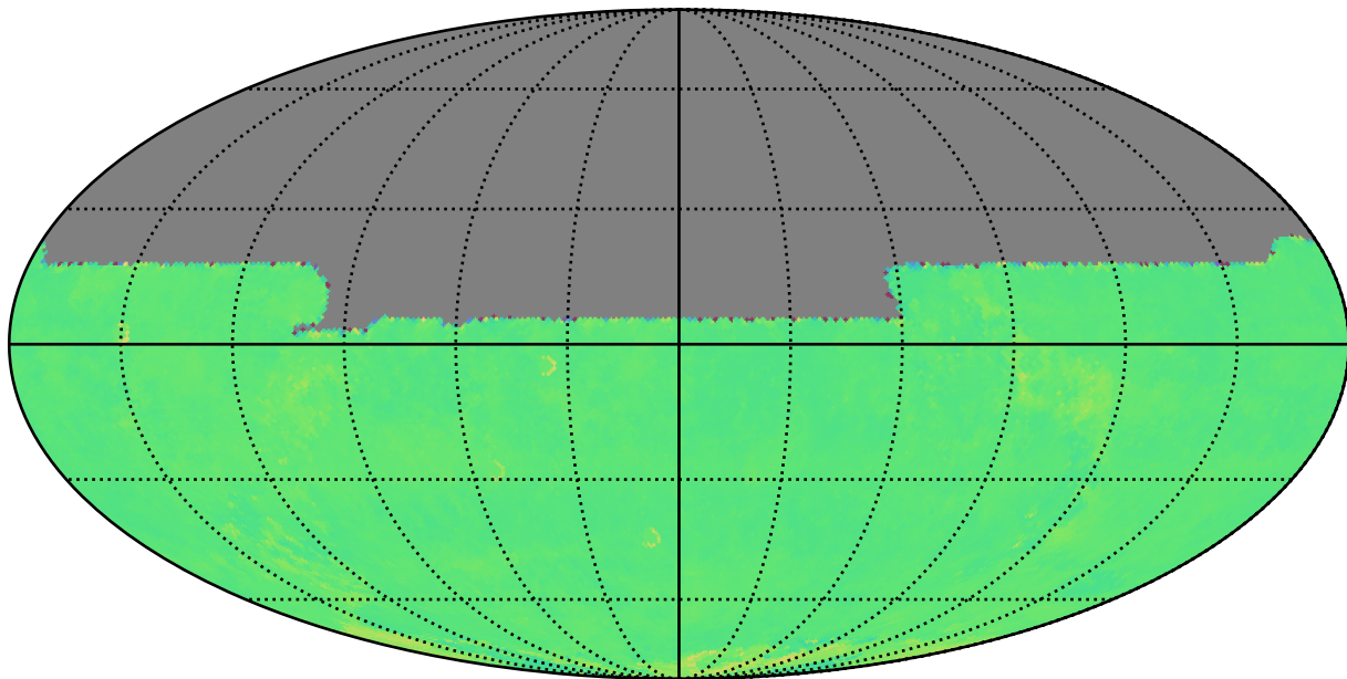
ddf_loaded_fl4_v3.4_10yrs y: Kuiper rotTelPos
