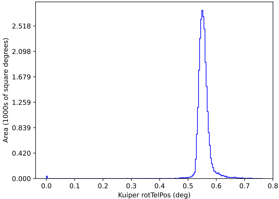
ddf_loaded_fl4_v3.4_10yrs y: Kuiper rotTelPos
