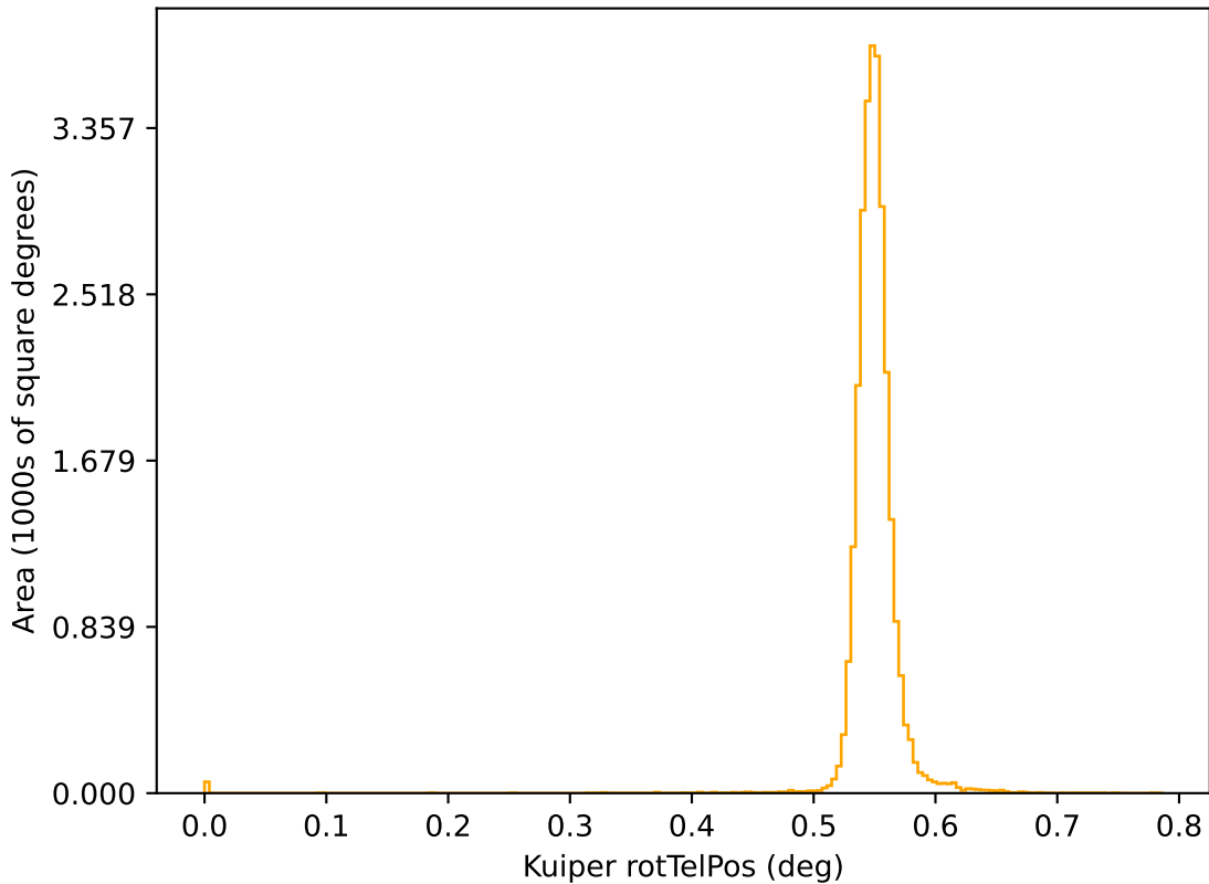
ddf_loaded_fl4_v3.4_10yrs r: Kuiper rotTelPos
