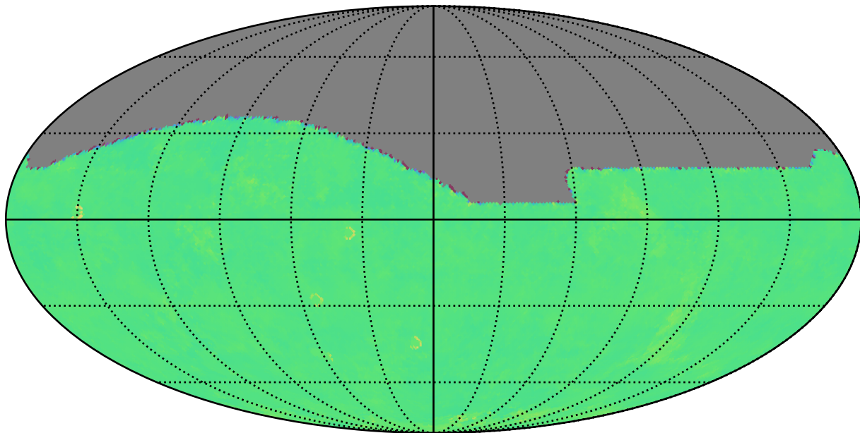
ddf_loaded_fl4_v3.4_10yrs i: Kuiper rotTelPos
