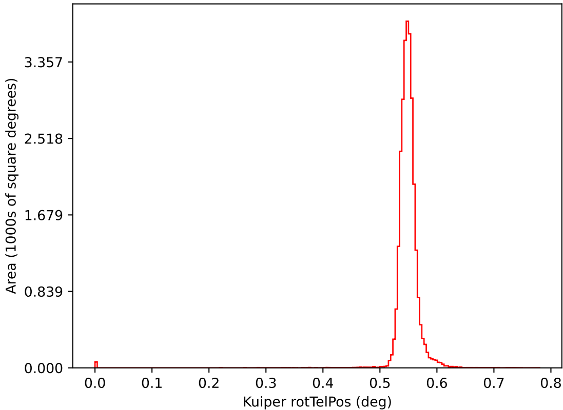
ddf_loaded_fl4_v3.4_10yrs i: Kuiper rotTelPos
