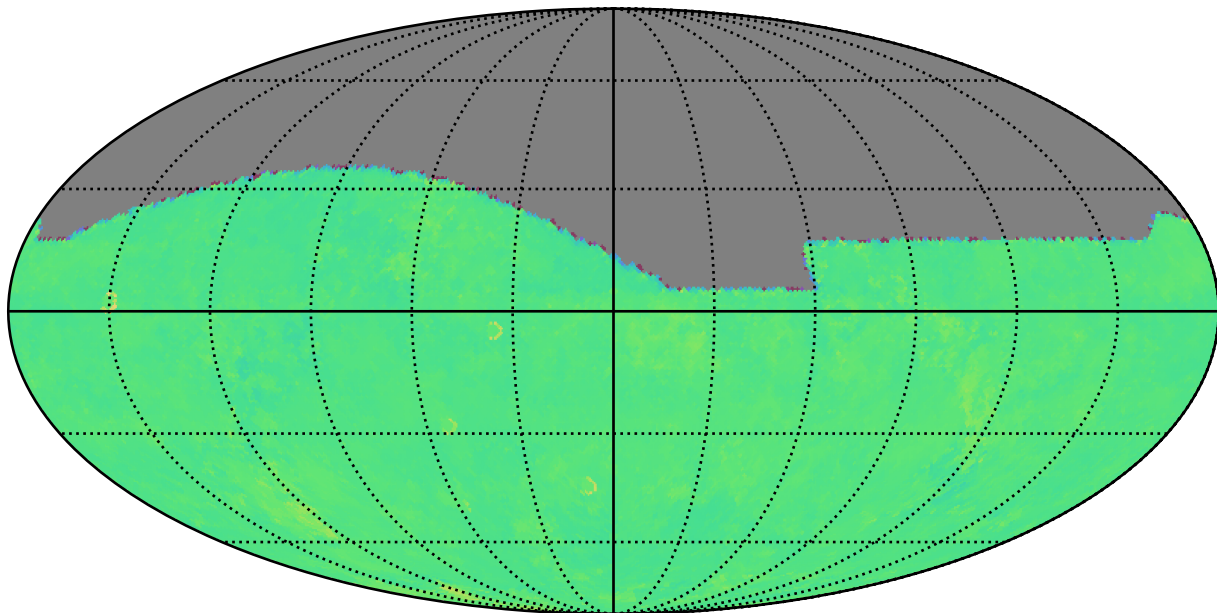
ddf_loaded_fl4_v3.4_10yrs g: Kuiper rotTelPos
