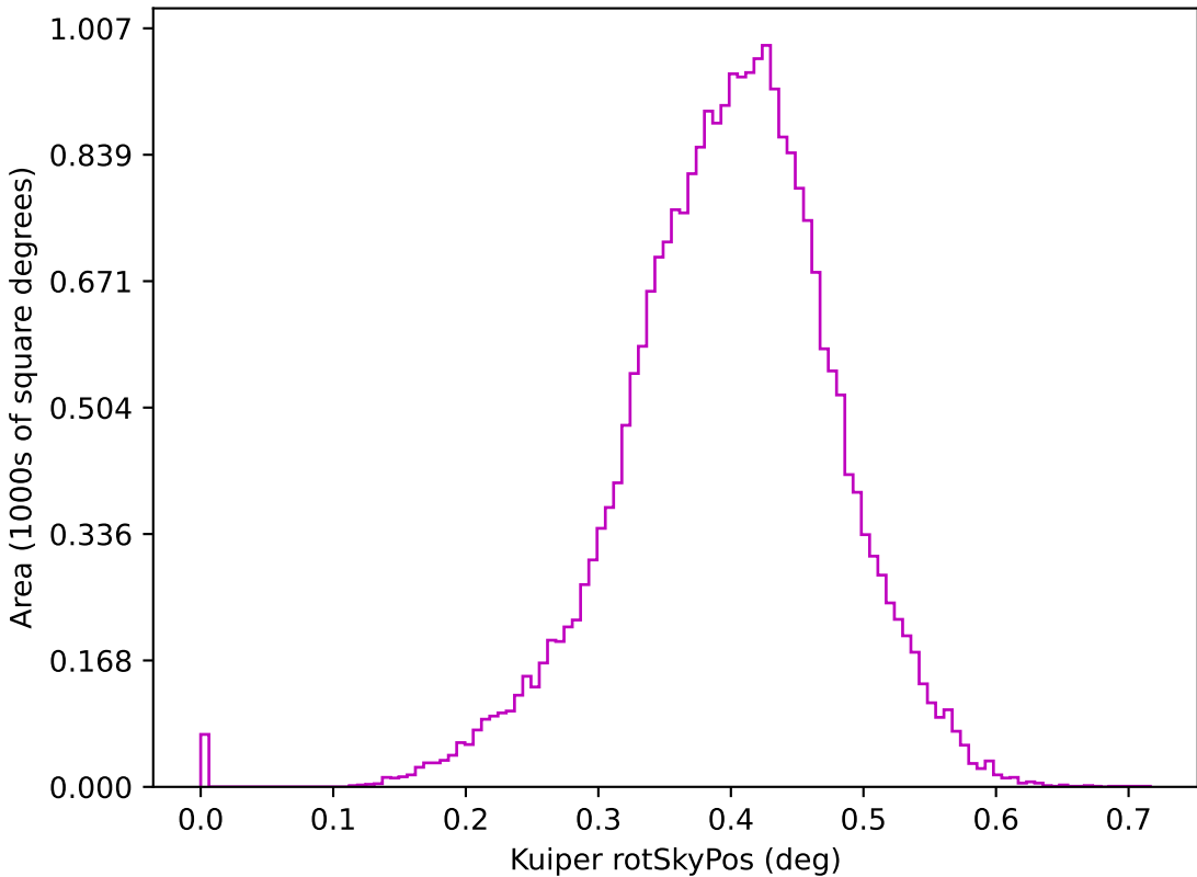
ddf_loaded_fl4_v3.4_10yrs z: Kuiper rotSkyPos
