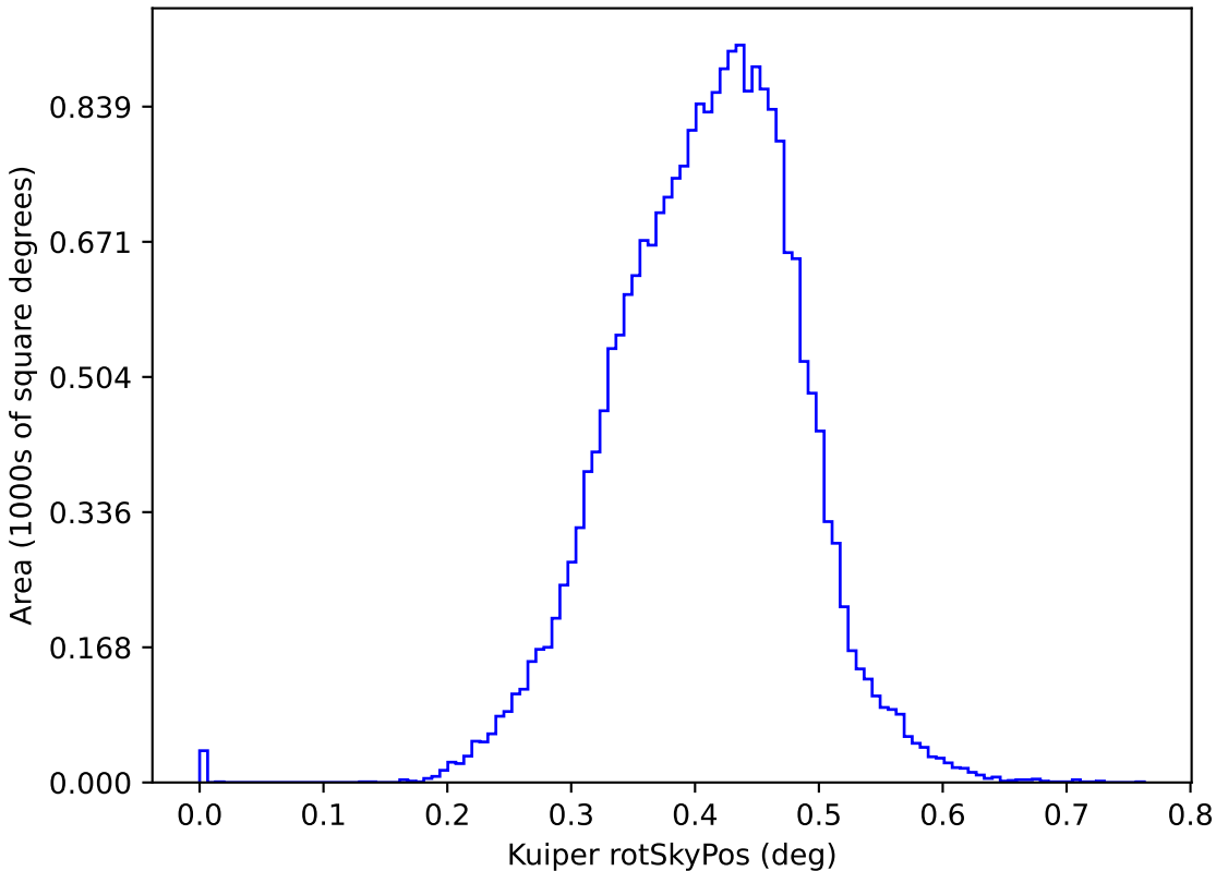
ddf_loaded_fl4_v3.4_10yrs y: Kuiper rotSkyPos
