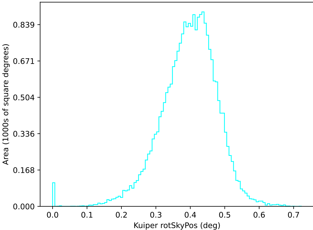
ddf_loaded_fl4_v3.4_10yrs u: Kuiper rotSkyPos
