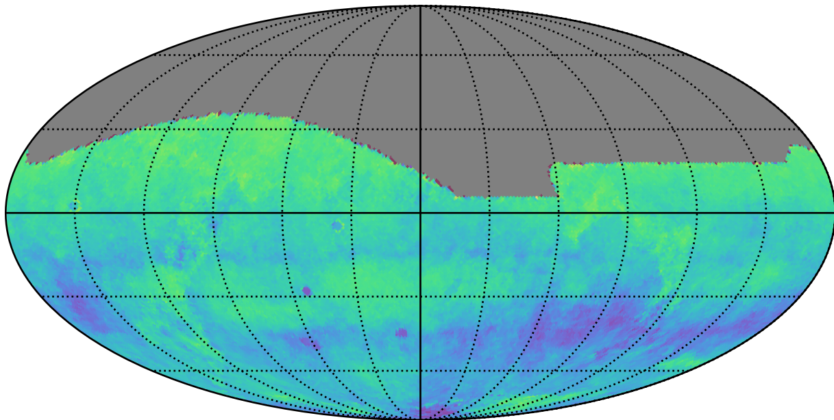
ddf_loaded_fl4_v3.4_10yrs i: Kuiper rotSkyPos
