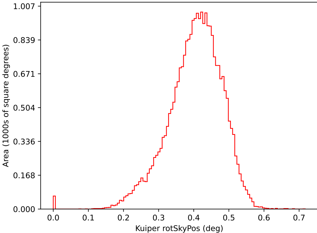
ddf_loaded_fl4_v3.4_10yrs i: Kuiper rotSkyPos
