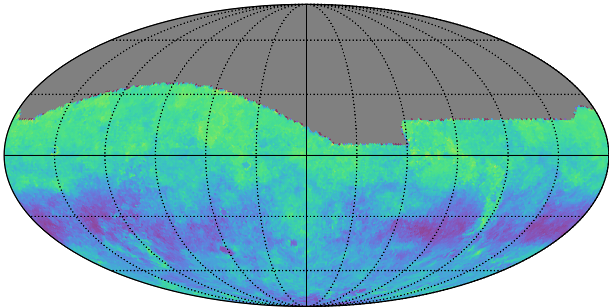
ddf_loaded_fl4_v3.4_10yrs g: Kuiper rotSkyPos
