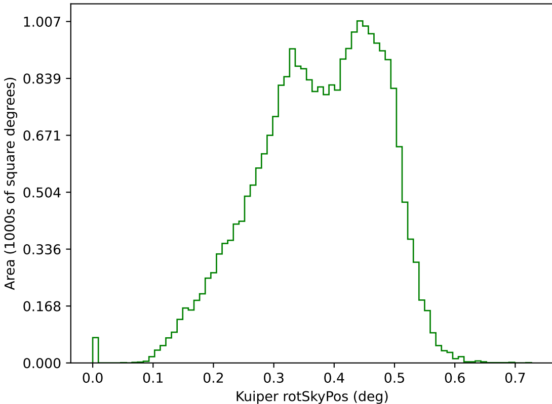
ddf_loaded_fl4_v3.4_10yrs g: Kuiper rotSkyPos
