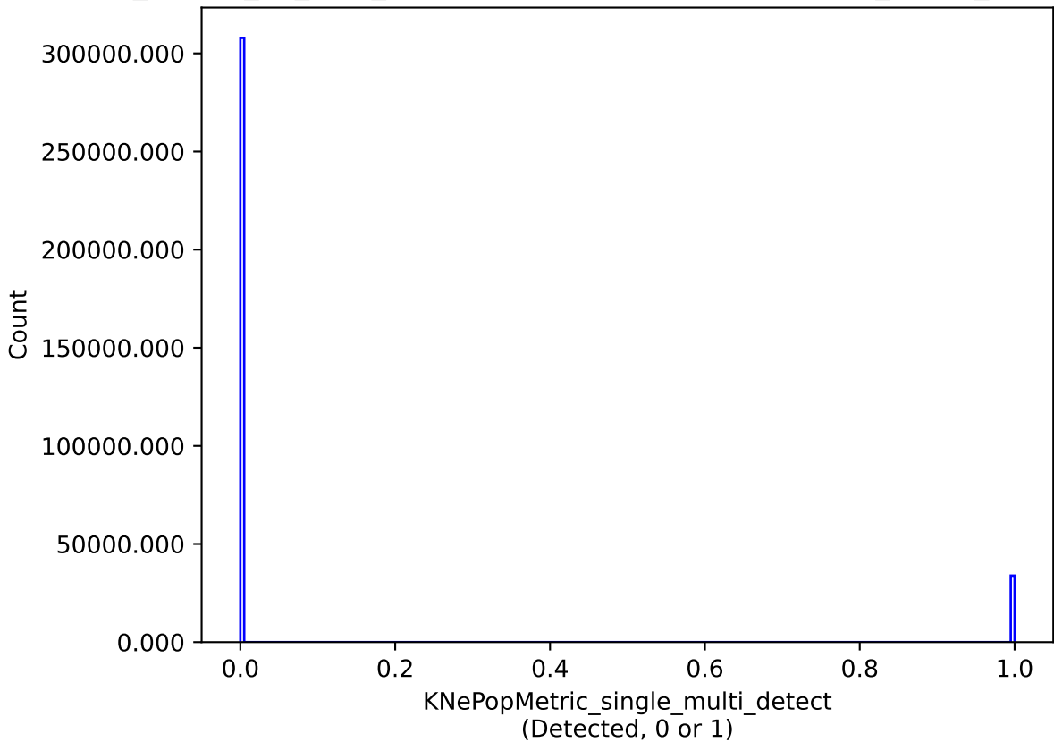
ddf_loaded_fl4_v3.4_10yrs single model: KNePopMetric_single_multi_detect
