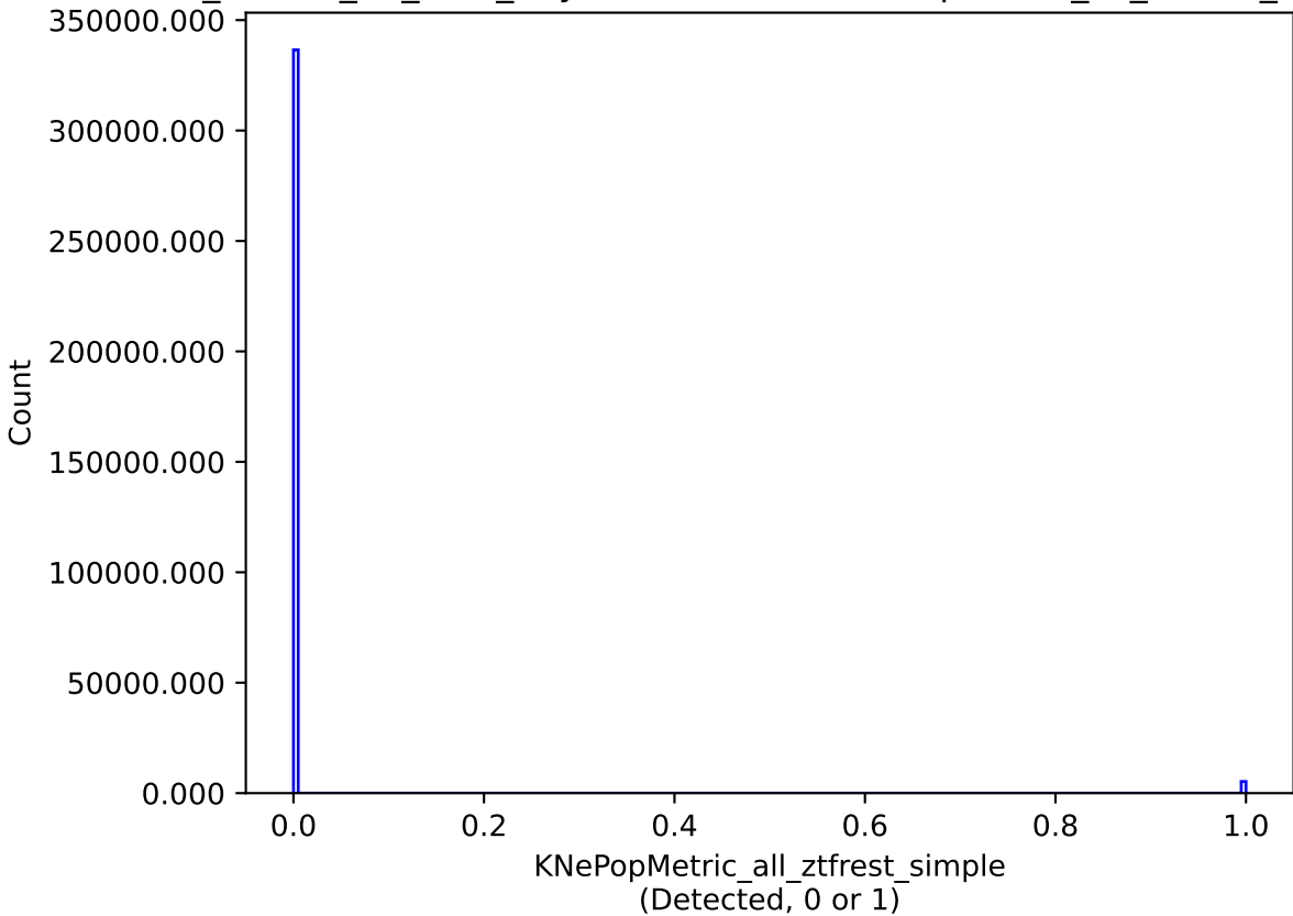
ddf_loaded_fl4_v3.4_10yrs all models: KNePopMetric_all_ztfrest_simple
