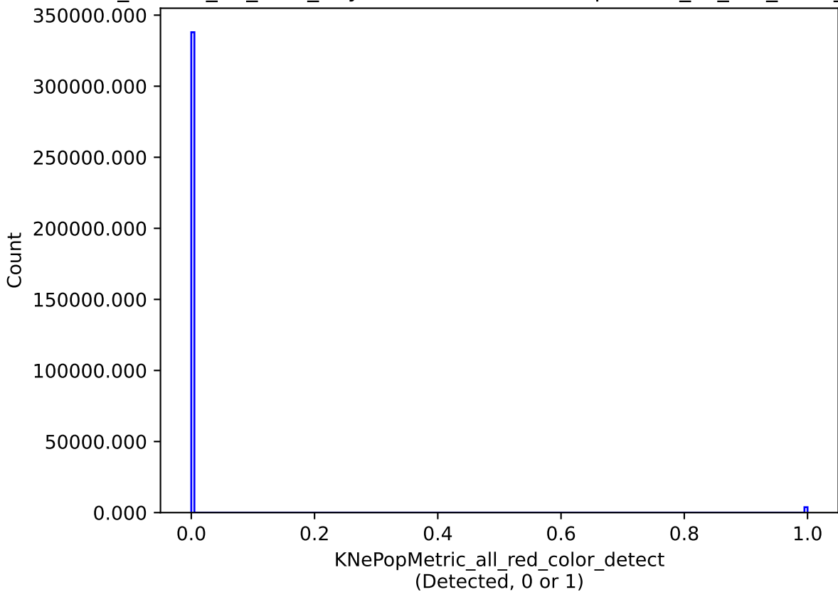
ddf_loaded_fl4_v3.4_10yrs all models: KNePopMetric_all_red_color_detect
