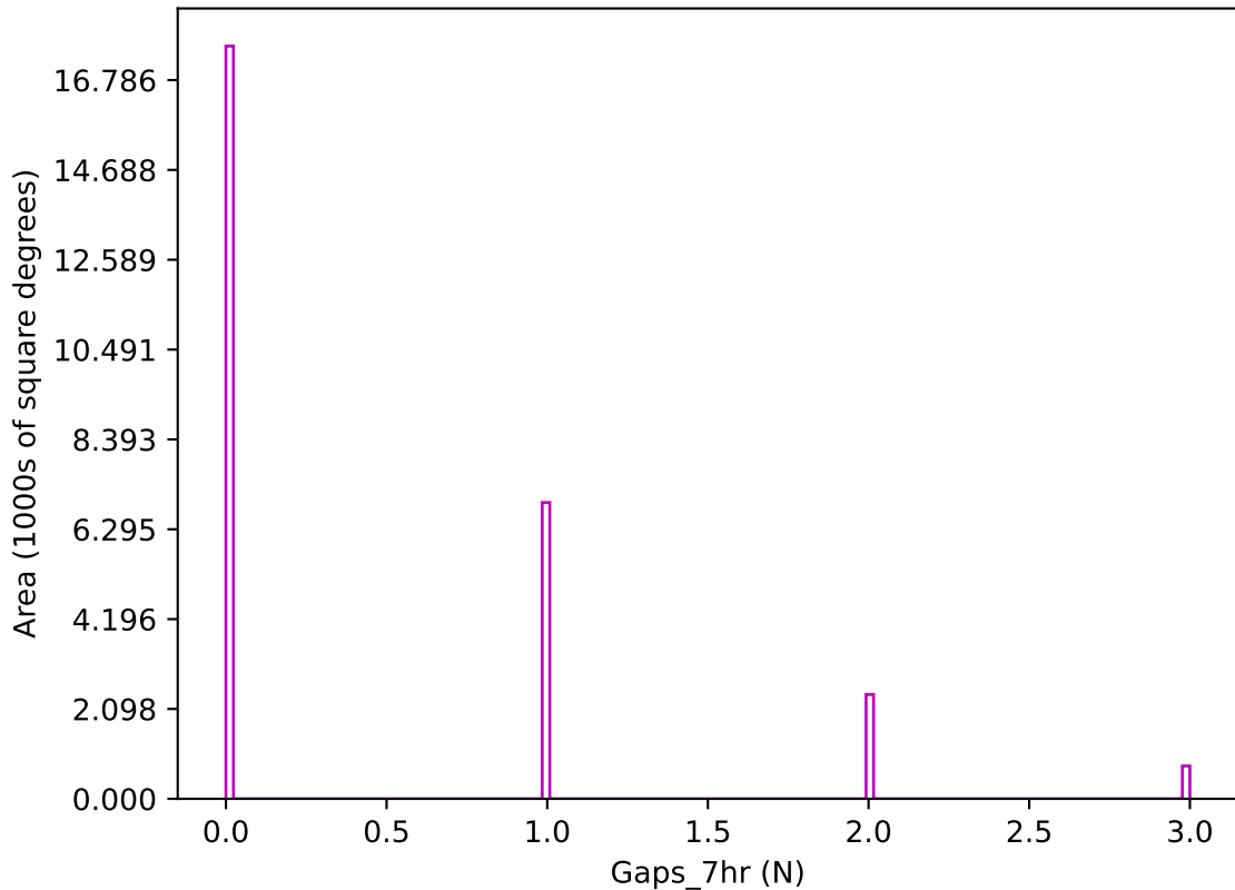
ddf_loaded_fl4_v3.4_10yrs z band: Gaps_7hr
