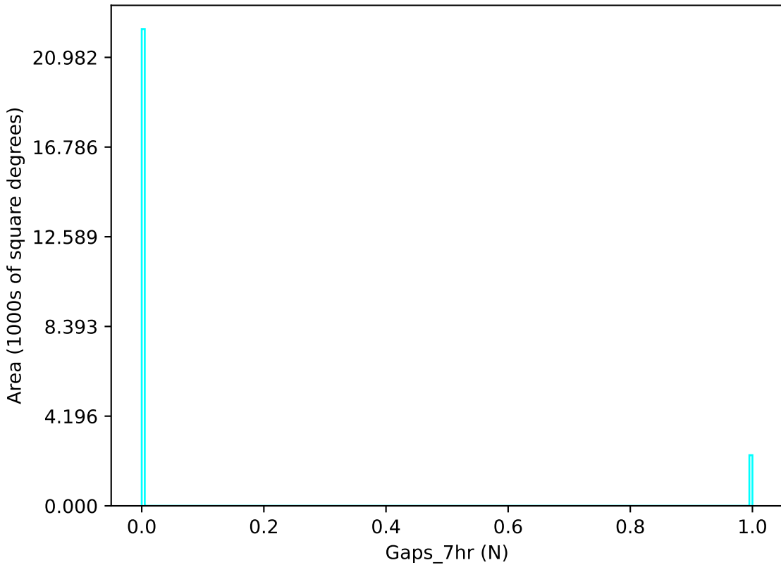
ddf_loaded_fl4_v3.4_10yrs u band: Gaps_7hr
