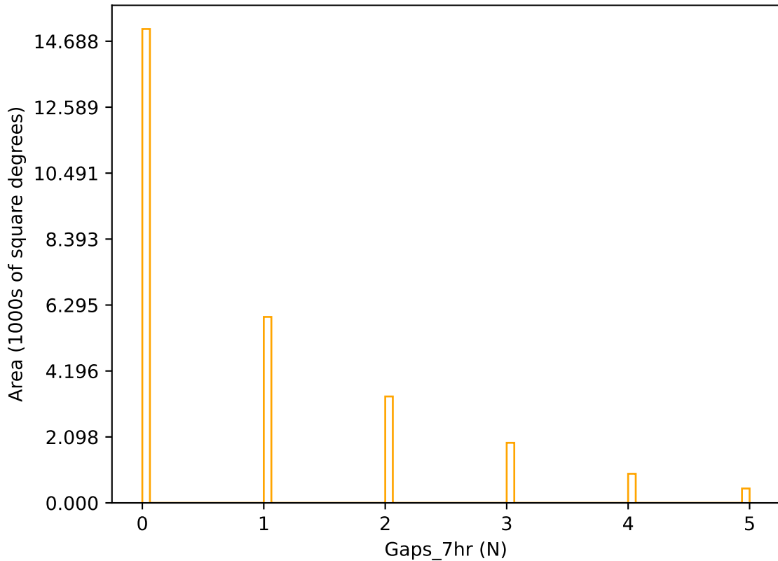
ddf_loaded_fl4_v3.4_10yrs r band: Gaps_7hr
