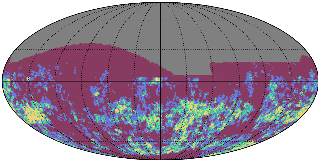
ddf_loaded_fl4_v3.4_10yrs i band: Gaps_7hr
