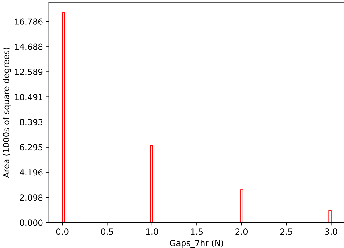
ddf_loaded_fl4_v3.4_10yrs i band: Gaps_7hr
